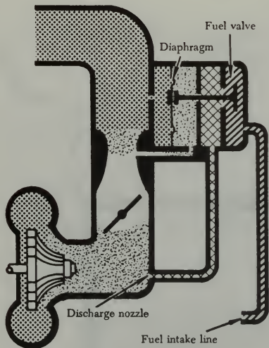
FIGURE 3-17. Pressure-type carburetor.
